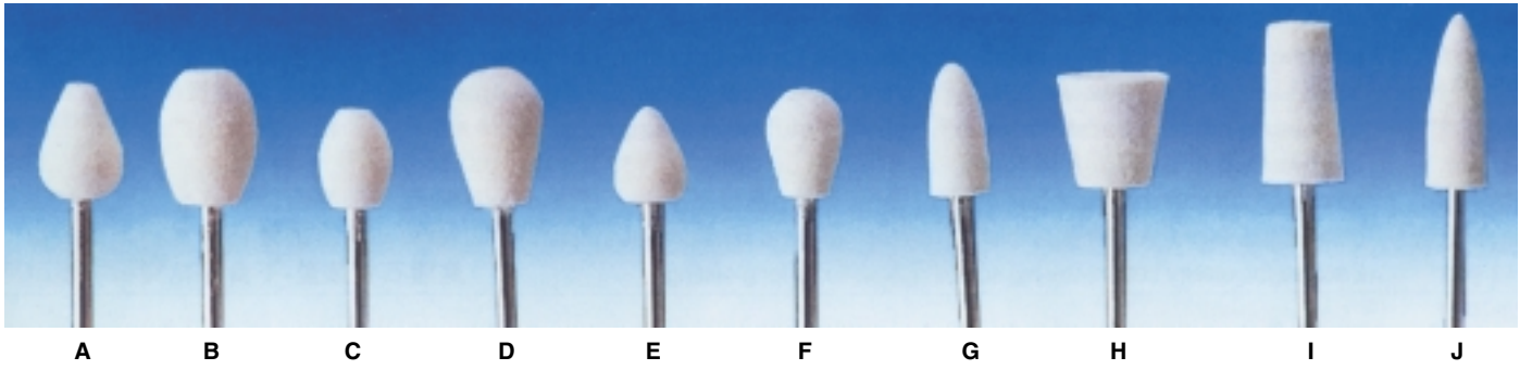
MOUNTED FELT POINTS
